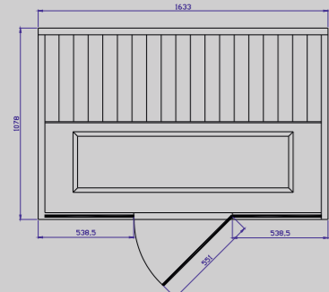
TYLÖSAND T-825 Dimensions: D 1078 x W 1633 mm Output: 1980 W
