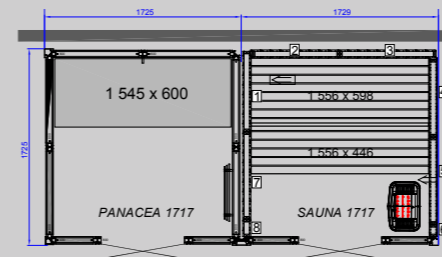
TWIN PANACEA 1717 Dimensions: D 1725 x W 3454 mm
