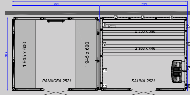
TWIN PANACEA 2521 Dimensions: D 2125 x W 5054 mm
