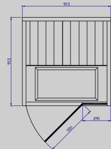
TYLÖSAND T-810 Dimensions: D 913 x W 913 mm Output: 1350 W
