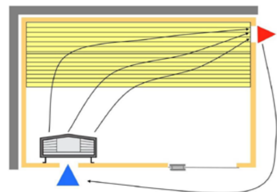
Properly ventilated sauna.
