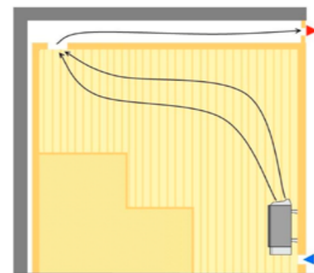
If the sauna ceiling is lowered, the space above can be used for ventilation.
