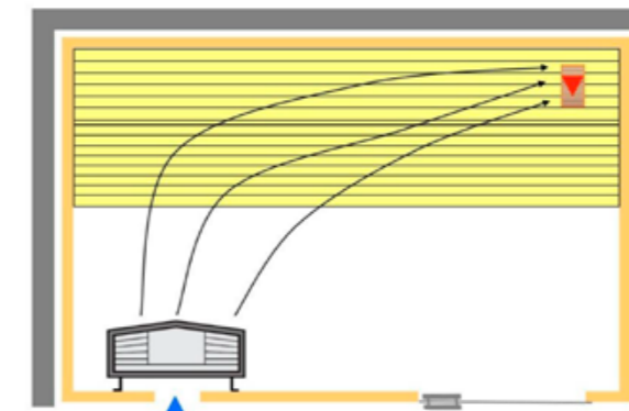
Make sure that the inlet and exhaust air openings are the same size, and that the air leaving the sauna flows into the same space from which the air is drawn in.
