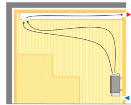
You can also solve the ventilation with a duct inside the sauna if there is no other option.
